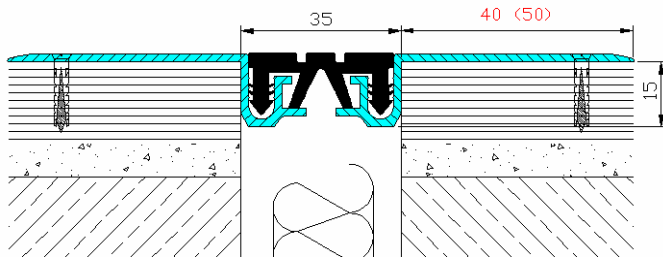
DL 1F 35*40 DL 1F 35*50
