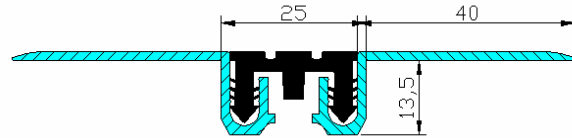
DL 1F 100*40 DL 1F 100*50 DL 1F 100*70
