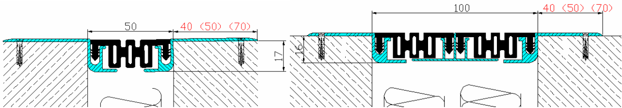
DL 1F 50*40 DL 1F 50*50 DL 1F 50*70
